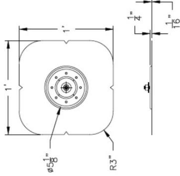
8 MECHANICAL ANCHOR DETAIL SCALE: 1-1/2" = 1'-0"
